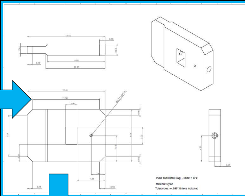
Nylon Push Tool
